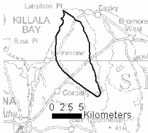
Figure 1 Location and Boundaries of Easky Left GWB.
