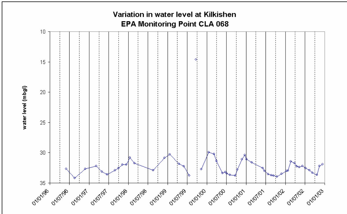
Figure 1: Groundwater hydrograph
